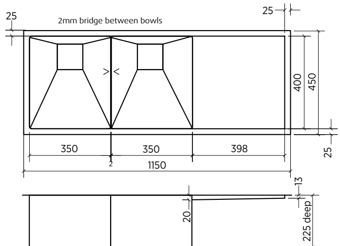
Undermount version has 25mm surround on all sides
